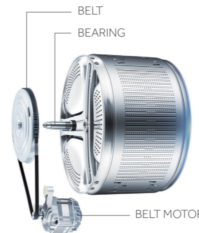
Inverter motor
